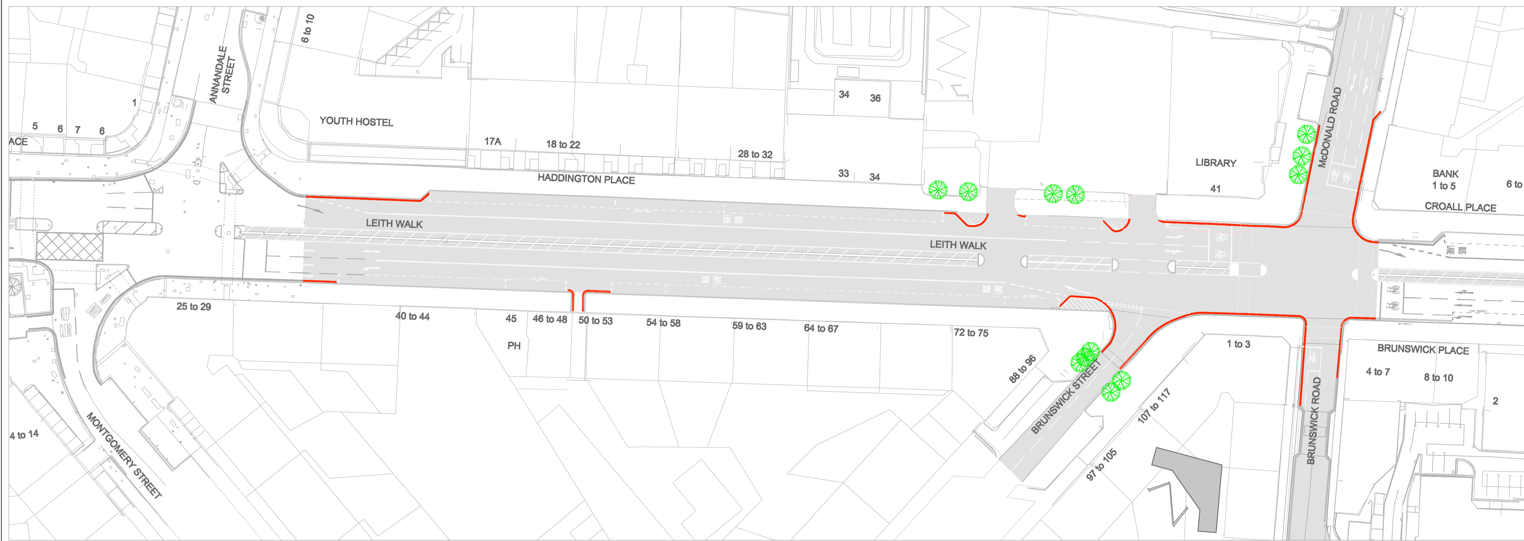
EXISTING LAYOUT OF LEITH WALK BETWEEN ANNANDALE STREET AND McDONALD ROAD (SECTION 3)
