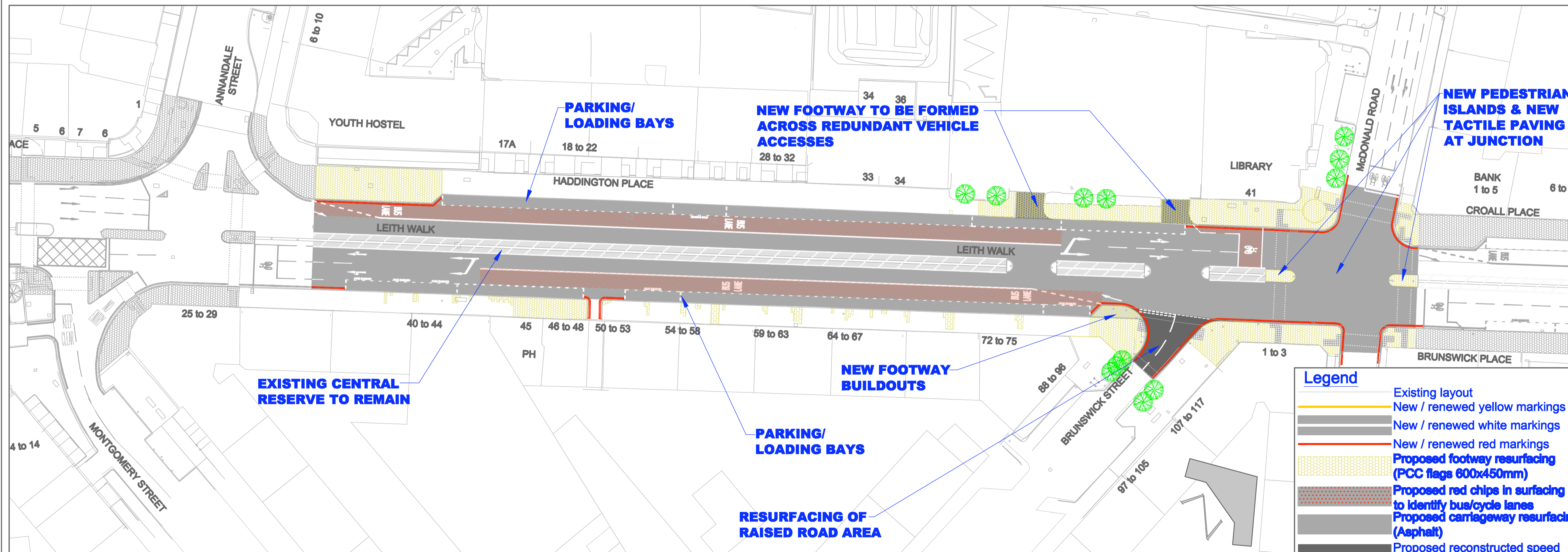
PROPOSED LEITH WALK IMPROVEMENTS BETWEEN ANNANDALE STREET AND McDONALD ROAD (SECTION 3)
