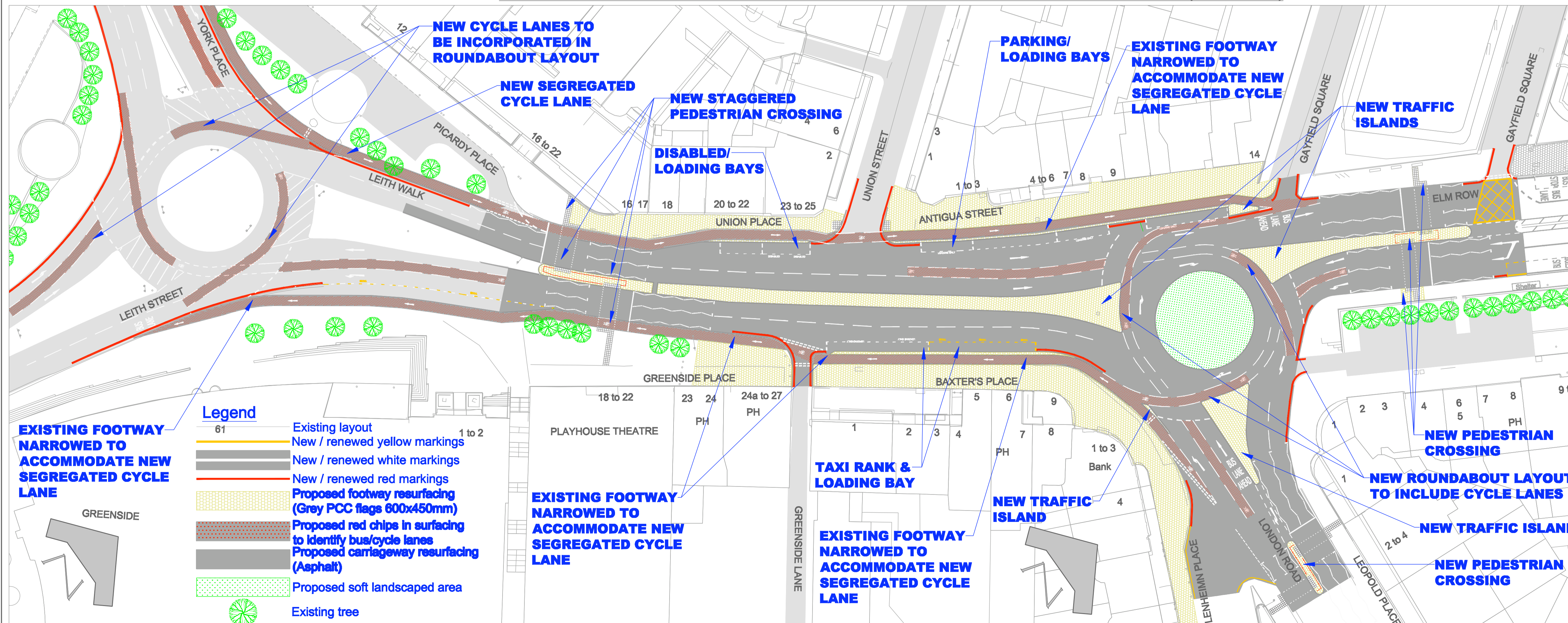
PROPOSED LEITH WALK IMPROVEMENTS BETWEEN PICARDY PLACE AND GAYFIELD SQUARE (SECTION 1)
