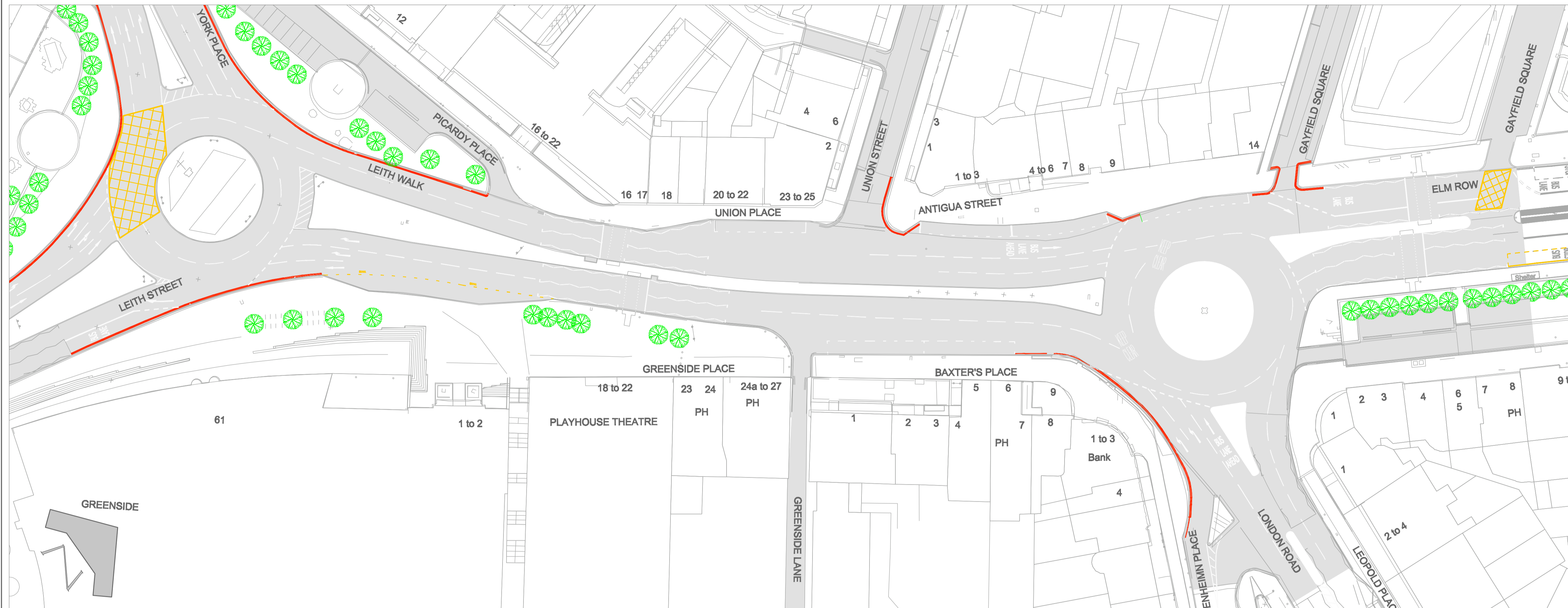
EXISTING LAYOUT OF LEITH WALK BETWEEN PICARDY PLACE AND GAYFIELD SQUARE (SECTION 1)
